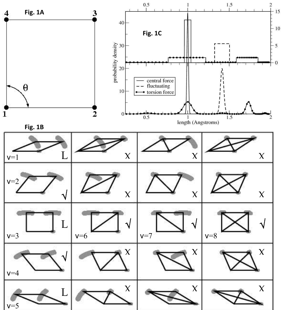
Fig. 1. (A) Definition of the quadrilateral network. (B) The accessible range of motion for each coarse-grained configuration is shown in grey. The middle two columns show how the more limited range of motion along a diagonal interaction compared to the range allowed by the torsion-forces is the determining factor restricting the motion. The symbols ( \checkmark , L, X) indicate which configurations are (very probable, improbable, inaccessible). The index, v , is used to label all accessible configurations. In the example considered here, the inaccessible configurations essentially have infinite energy, but in a more refined model they could have a finite energy. (C) Treating interactions as independent , the probability density, \rho(\ell) , for the length of a distance constraint is plotted for central-, fluctuating- and torsion-interactions, where the lower and upper graphs correspond to the cases: g = 8 kcal/mol and g = 0 .
