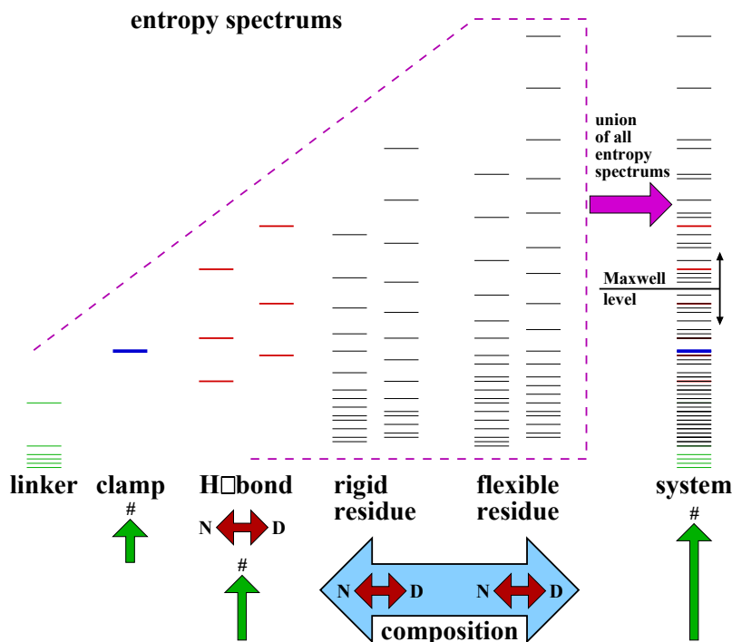
Fig. 7. Schematic of how the entropy spectrums associated with subsystems combine into a single entropy spectrum for the entire system. Green vertical arrows pointing to the # sign indicate that the number of interactions depend on the decorated microstate. The “clamp” interaction derives from clathrate water. The horizontal dark red double arrow indicates a certain number of interactions can be native like (N) or disordered (D), and their respective entropy spectrums are shown. Each residue has a unique entropy spectrum. Residues with (smaller, larger) entropy values are more (rigid, flexible). The protein sequence defining the residue composition is represented as the large horizontal blue double arrows. The system entropy spectrum is characterized by the variables ( p_c , q_c ). From Eq. (20) distance constraints with entropy less than the Maxwell level are independent, and this level slides up and down the spectrum depending on numbers and types of interactions present in the system.
