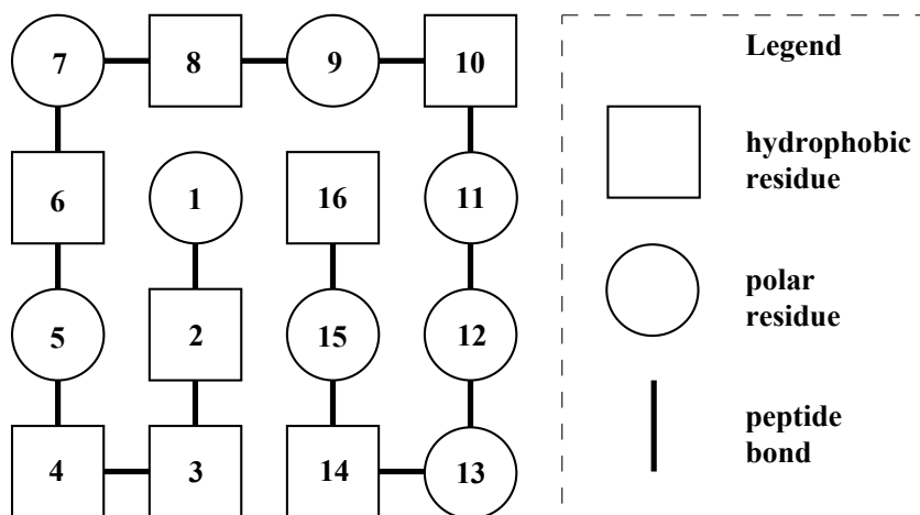
Fig. 4. A schematic of a protein template structure is shown consisting of 16 residues. Each residue defines a subsystem that includes all atoms from its backbone and sidechain. The model can include a sufficient number of probable low energy basins for each residue type covering the most frequently occurring conformations identified in the Ramachandran plot and the sidechain rotamers. The degree of coverage depends on the level of coarse graining, which ultimately controls the accuracy of the model and speed of the calculations.
