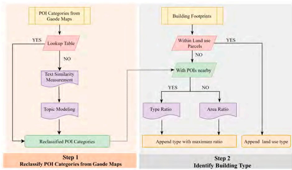
Figure 3. The proposed framework for identifying building types.
