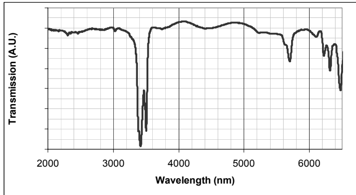
Figure 6. Transmission spectrum of the FLC cell.
