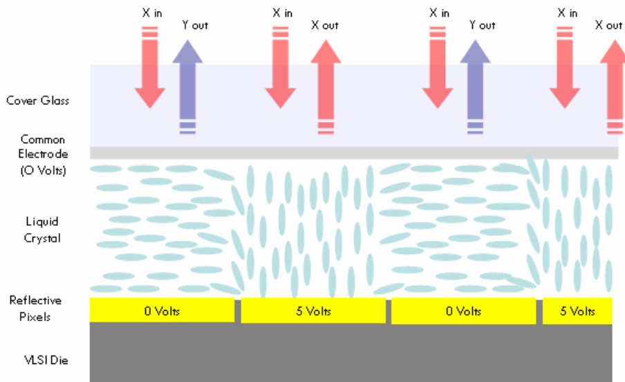
Figure 1. Side view of a LCOS display.
