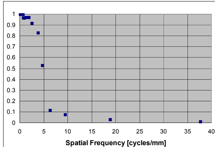
Figure 4. Measured MTF of the UCF nematic display.
