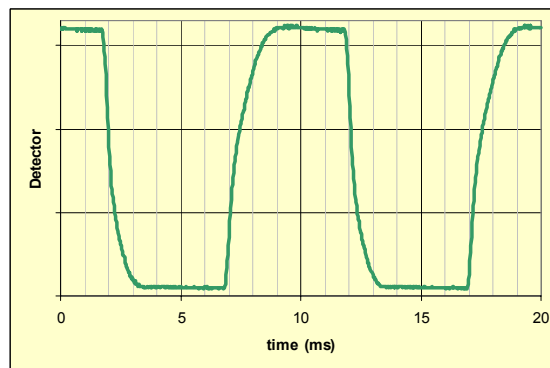
Figure 5. Switching response of the MWIR FLC cell.
