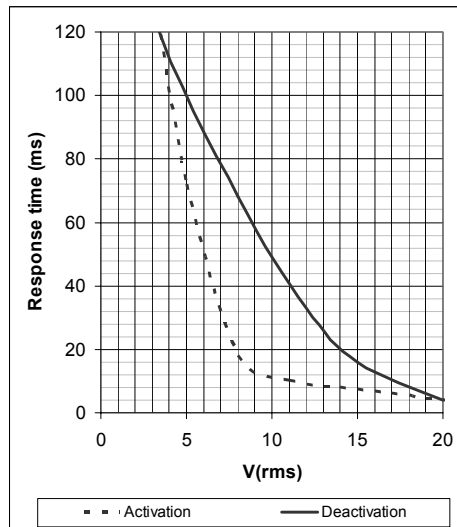
Figure 7. Response time of the MWIR Dual-Frequency nematic cell.
