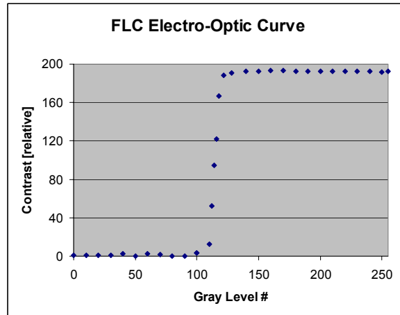
Figure 8. Grayscale response of the FLC display.
