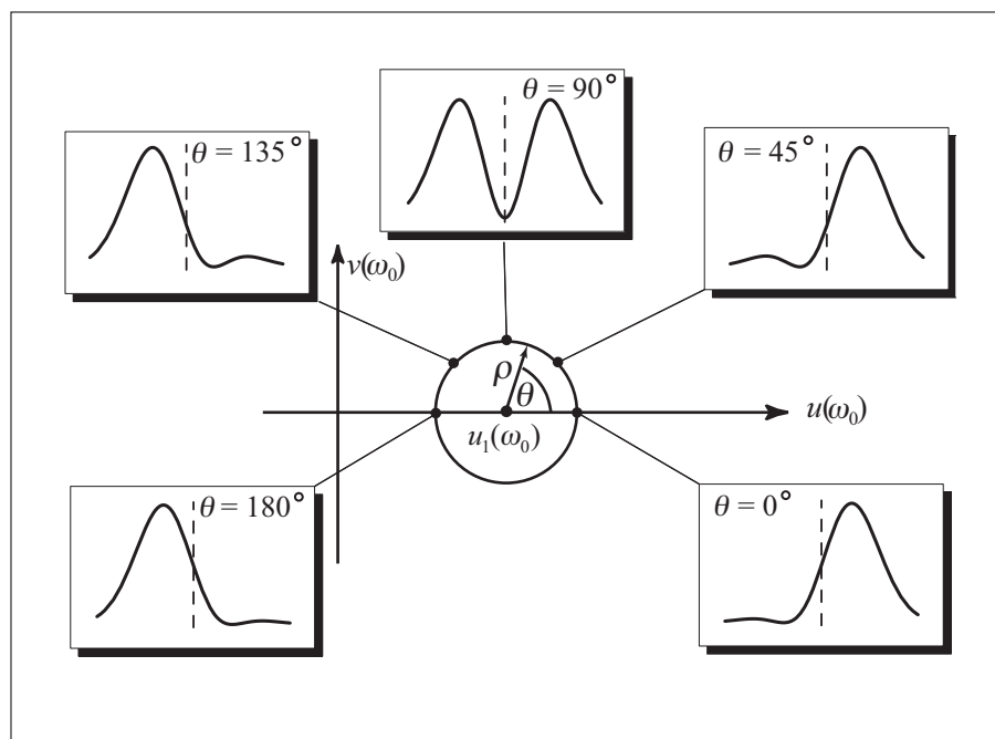
Figure 1. Schematic illustration of the spectrum along a loop encircling the first axial zero of the center frequency. [After G. Gbur, T. D. Visser and E. Wolf, Phys. Rev. Lett. 88 013901 (2002).]
