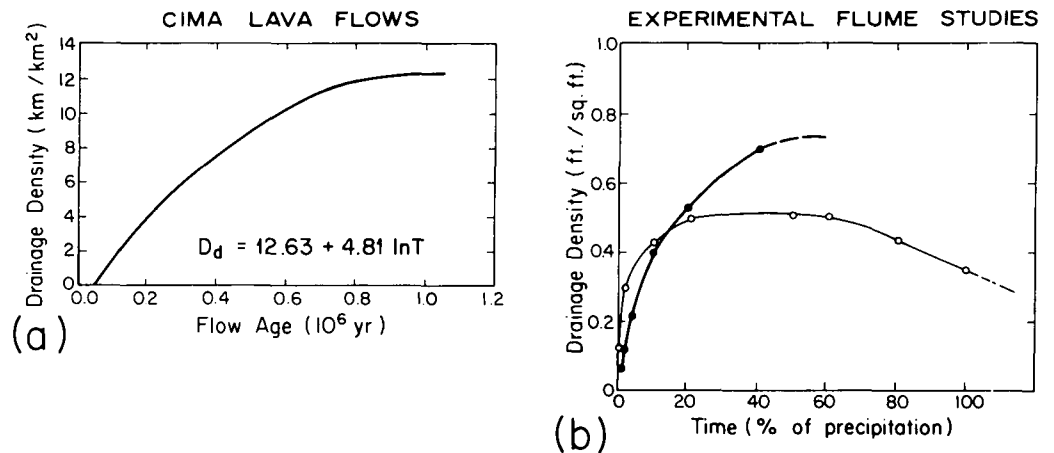
Figure 12. a. Age-dependent trend shown by best-fit curve in drainage density on basaltic flows using data in Figure 4. b. Drainage density changes during two flume experiments (after R. S. Parker, unpub. data).
