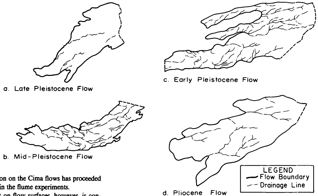
Figure 11. Drainage networks for selected flows dating from Pliocene to late Pleistocene. Note increasing drainage texture on progressively older flows and decrease in texture on Pliocene flow. Scale approximately equal in all frames, ~1:22,000.
