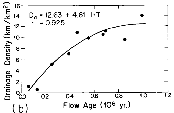
Figure 4. a. Drainage frequencies ( D_f ) for field measurements made on dated flows of different ages ( T ); solid line is statistically significant best-fit curve. b. Drainage densities ( D_d ) for dated flows of different ages ( T ); solid line is statistically significant best-fit curve.
