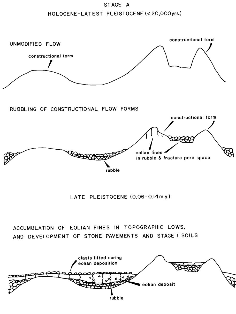
Figure 9. Schematic topographic and stratigraphic sections of late Cenozoic basaltic lava flows illustrating stages of flow-surface modification. Evolution of basaltic flow surfaces: Stage A: accretionary mantle deformation on flow surfaces by weathering and colluviation of bedrock topographic highs and by eolian deposition in topographic lows. Stage B: flow-surface stability; decreased weathering, colluviation, and eolian deposition; increased
